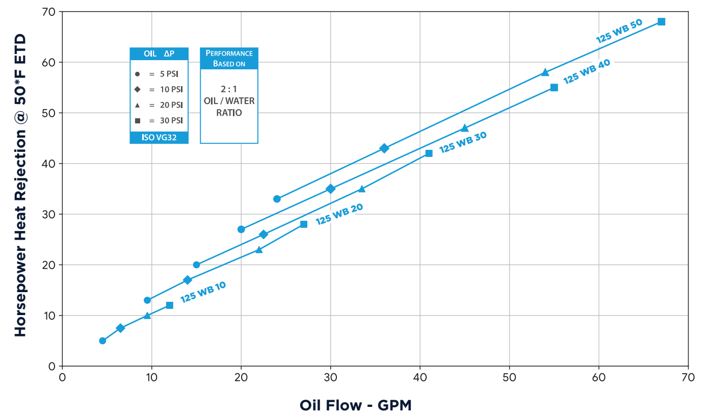
PERFORMANCE CHART
