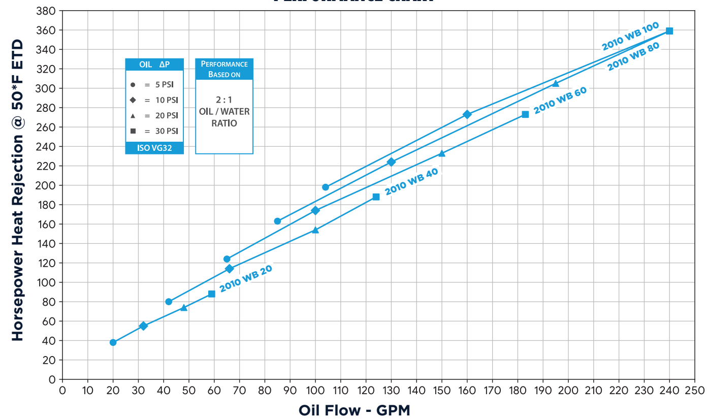
PERFORMANCE CHART
