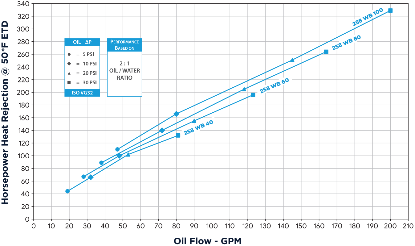
PERFORMANCE CHART
