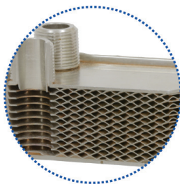
Cutaway to show high density, compact brazed plate construction
